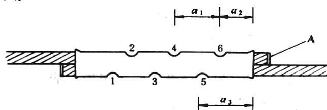
(I) LJ-35 铝绞线
